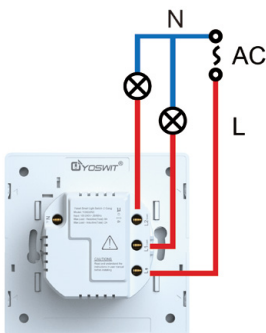
Connection 1: Without neutral wire
