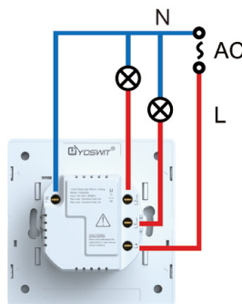
Connection 2: With neutral wire
